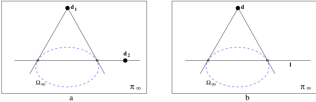
Fig. 3.8. Orthogonality and \Omega_\infty . (a) On \pi_\infty orthogonal directions d_1, d_2 are conjugate with respect to \Omega_\infty . (b) A plane normal direction d and the intersection line l of the plane with \pi_\infty are in pole–polar relation with respect to \Omega_\infty .
