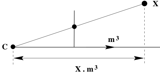
Fig. 6.6. If the camera matrix P = [M \mid \mathbf{p}_4] is normalized so that \|\mathbf{m}^3\| = 1 and \det M > 0 , and \mathbf{x} = w(x, y, 1)^T = P\mathbf{X} , where \mathbf{X} = (X, Y, Z, 1)^T , then w is the depth of the point \mathbf{X} from the camera centre in the direction of the principal ray of the camera.
